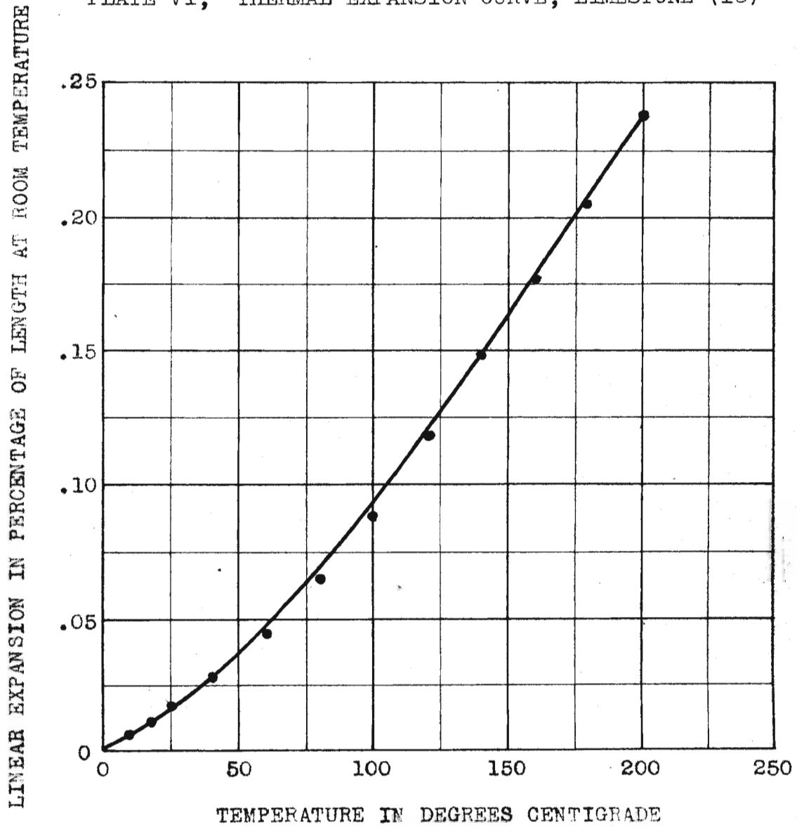
PLATE VI, THERMAL EXPANSION CURVE, LIMESTONE (18)
